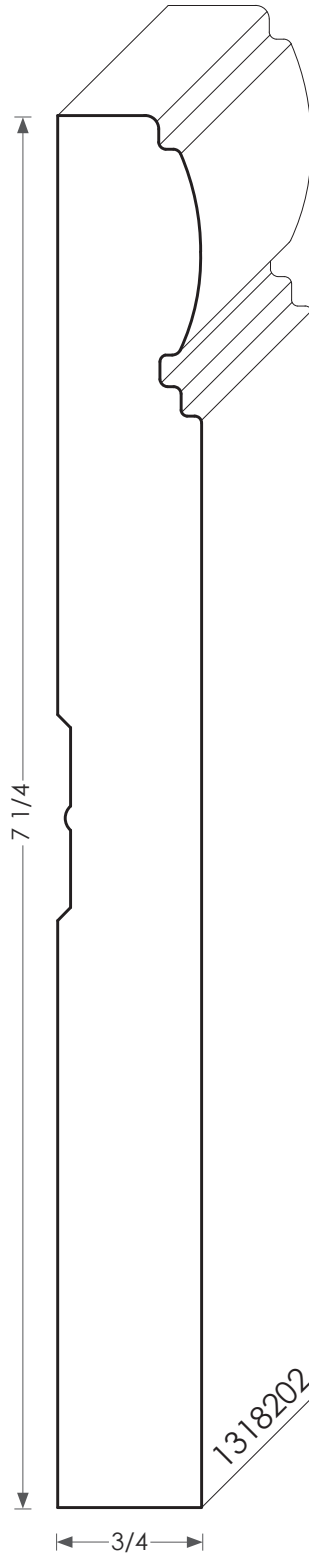
MDF Baseboard - 1318202
