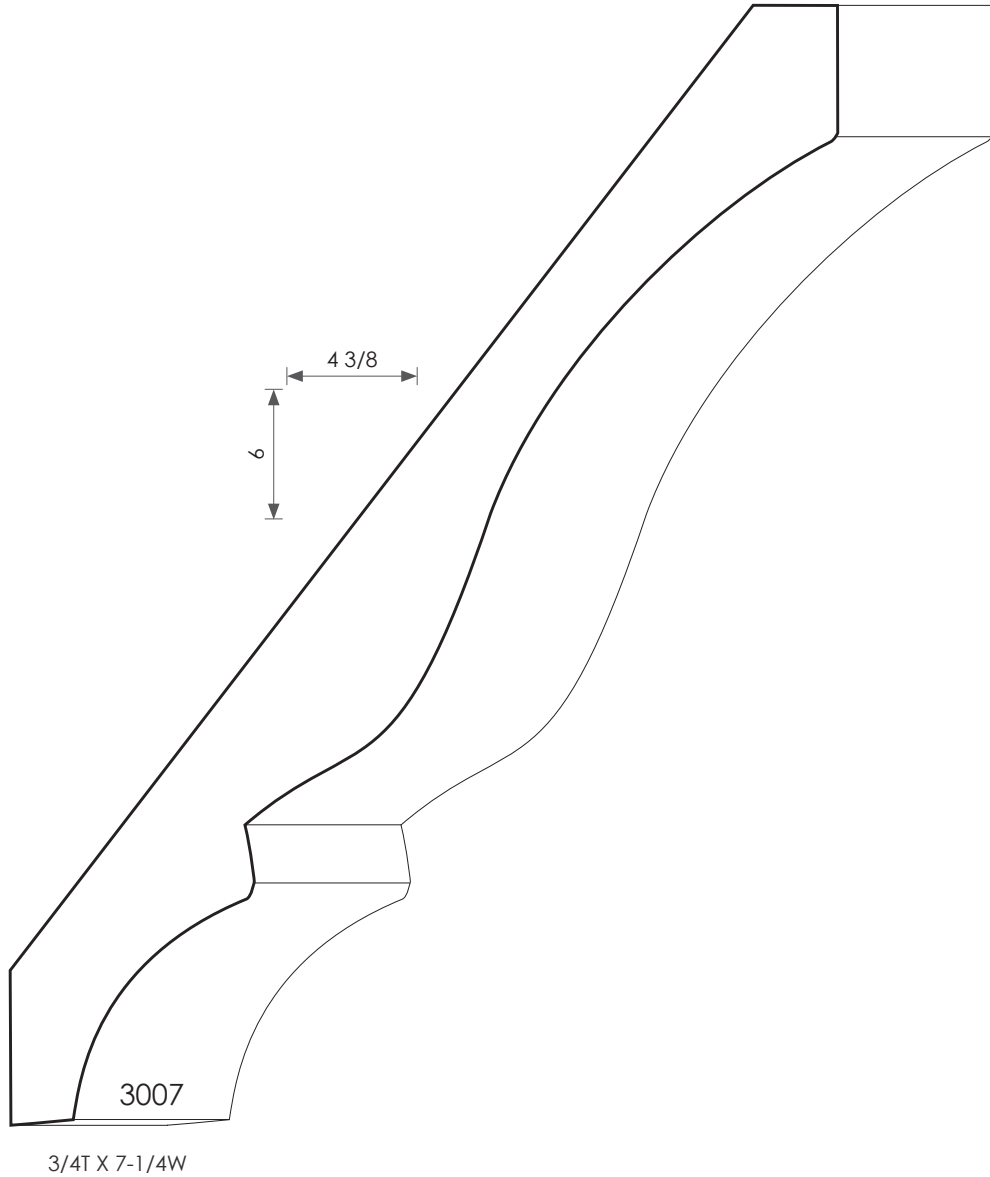
Wood Crown Mold - 3007
