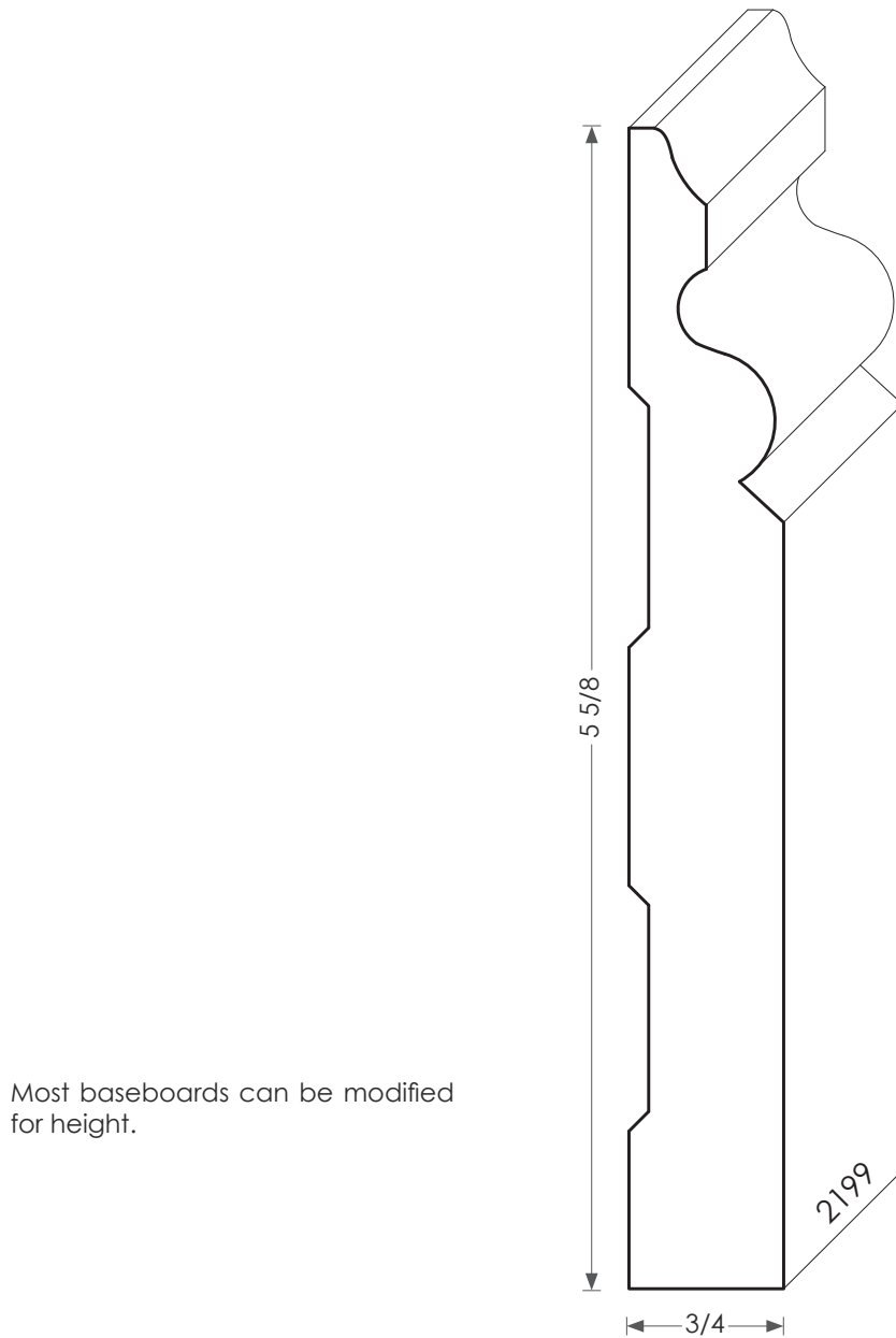
Wood Baseboard - 2199
