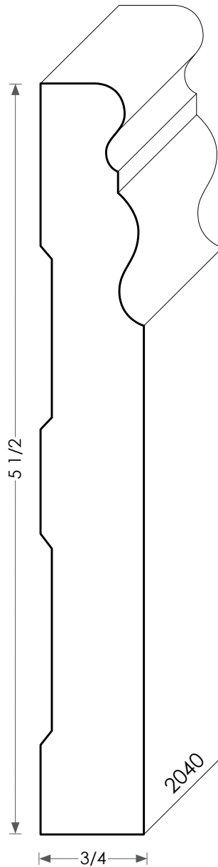
Wood Baseboard - 2040
