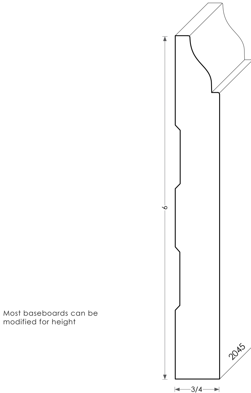
Wood Baseboard - 2045
