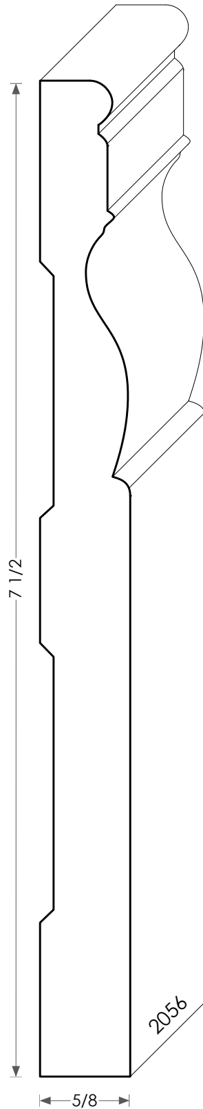
Wood Baseboard - 2056
