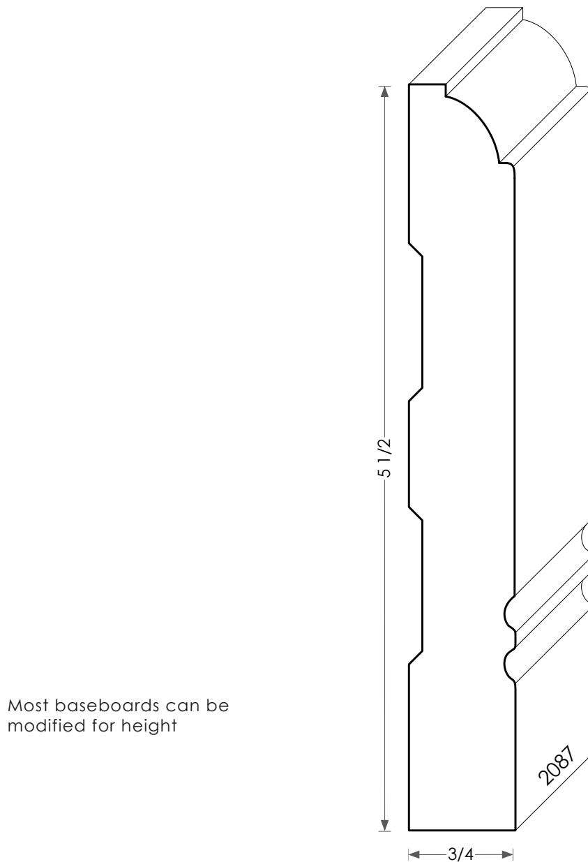
Wood Baseboard - 2087
