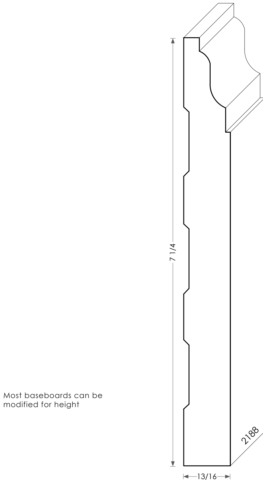
Wood Baseboard - 2188
