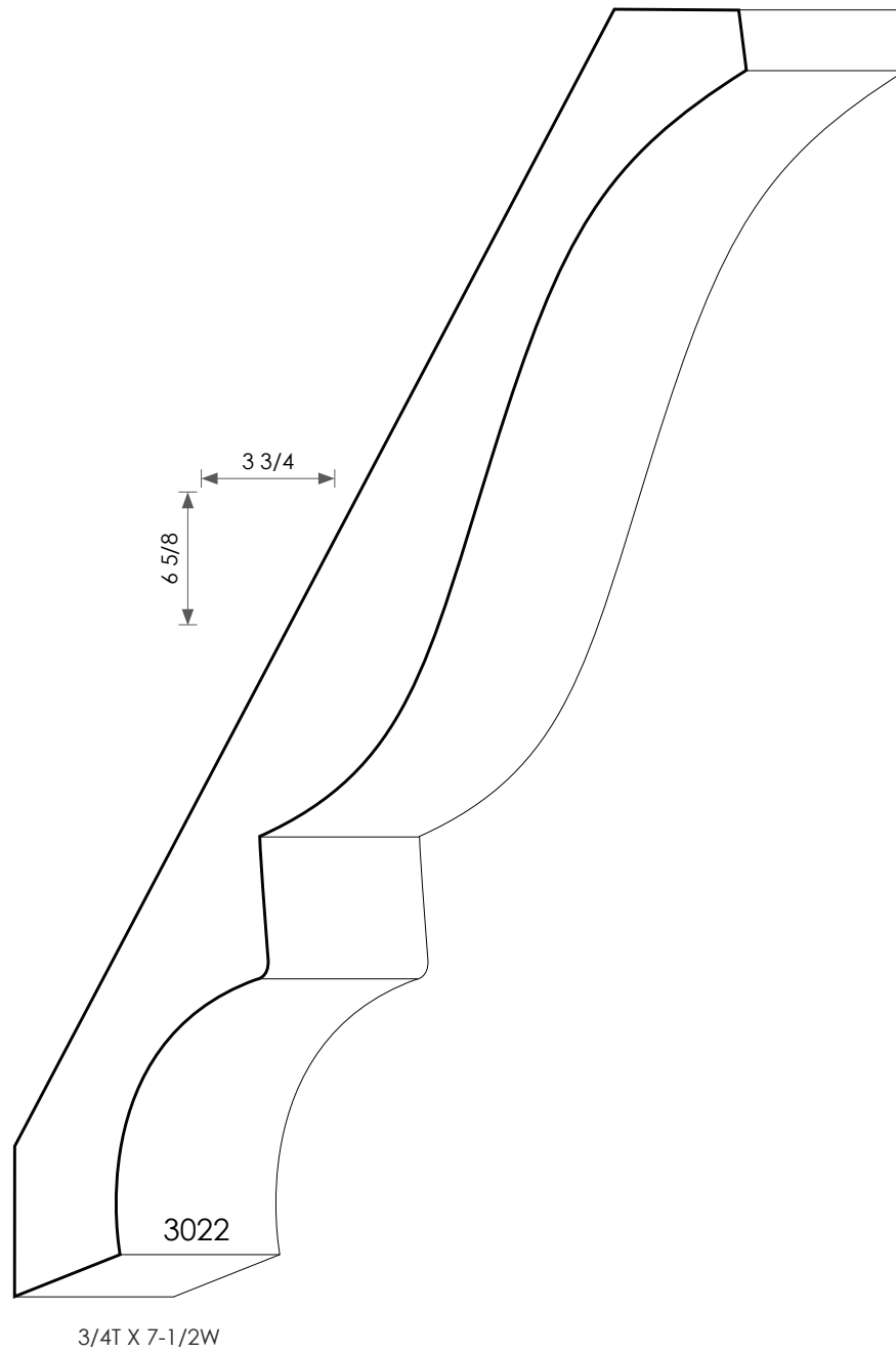
Wood Crown Mold - 3022
